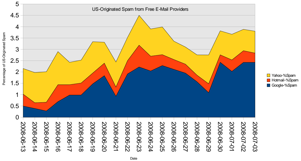
Figure 1: Percentage of US Spam Originating from Free E-Mail Providers
