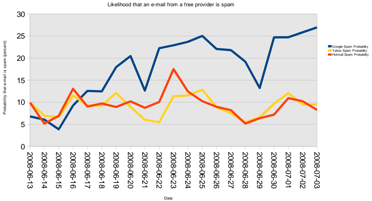
Figure 2: Likelihood that an E-Mail Originating from a Free Provider is Spam
